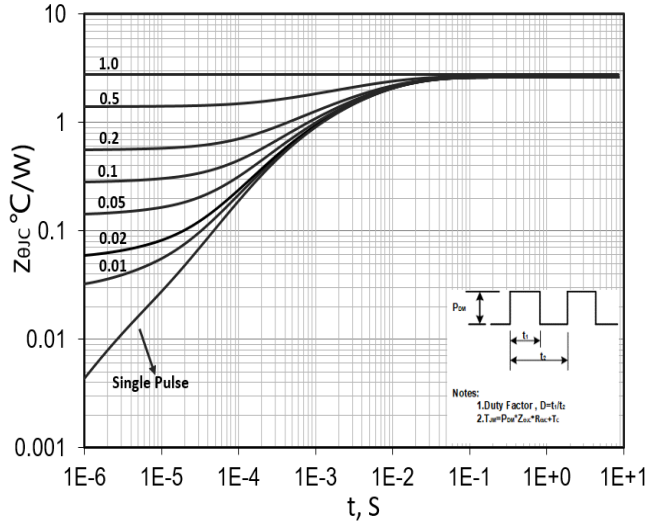
Figure 14. Transient Thermal Response Curve (TO-220F)
