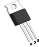
TO-220
