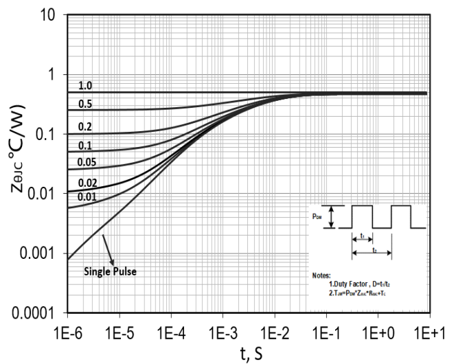
Figure 12. Transient Thermal Response Curve (TO-220)
